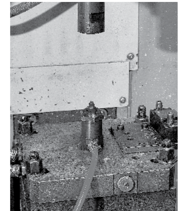
Centring pin made of CERAZUR in a complete electrode
