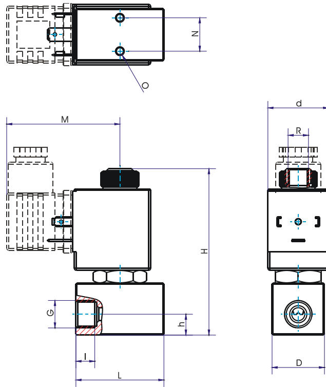
dimension table for type 84 in mm, weight approx. in g
